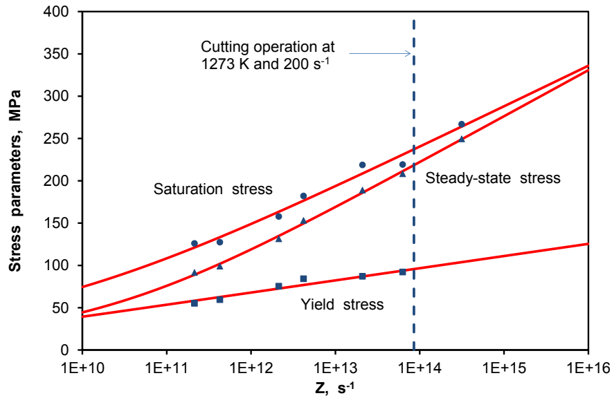
Figure 13: \sigma_y , \sigma_{sat} and \sigma_{ss} as a function of Z .
