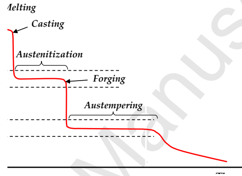
Figure 1: Heat treatment example for austempered ductile iron.
