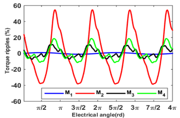
Fig. 8. Torque ripples calculated by FE simulations normalized with respect to the mean value for each operation mode.
