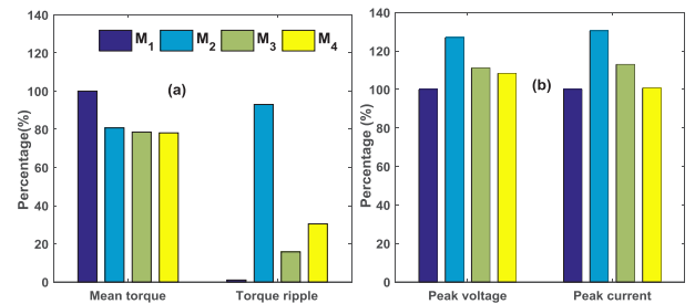
Fig. 7. Parameters of comparison between the healthy mode control strategy and post-fault control strategies.
