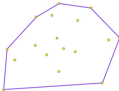
Figure 6. Two-dimensional (2D) convex hull structure for a given set of points.
