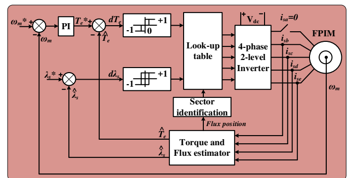
Fig. 3. DTC control scheme regulating the five-phase induction motor (FPIM) drive in open-phase fault situation.
