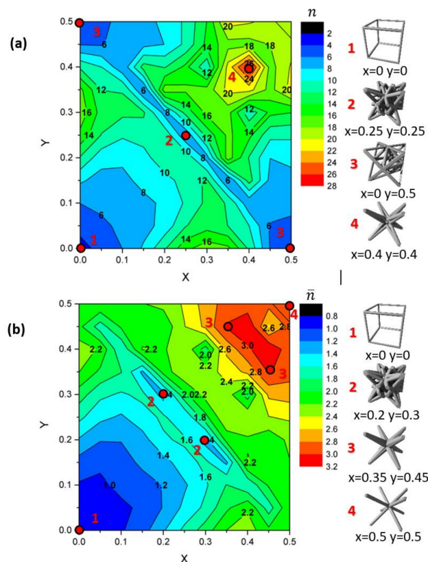
Figure 6. Parameter n indicating the dependence of the stress concentration factor on density for: (a) K = \sigma_m / \bar{\sigma} and (b) \bar{K} = \bar{\sigma} / \bar{\sigma} . The optimal solutions to maximize the yield stress are highlighted in red and the solutions to minimize it are indicated in blue.
