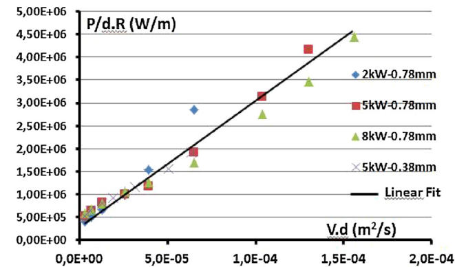
Fig. 1. For St35 steel and different operating parameters (incident powers and focal spot diameters), plot of P/(d \cdot R) as a function of the parameter V \cdot d and corresponding best linear fit (KH depths obtained by Suder and Williams, (2014) at 1.06 \mu\text{m} laser wavelength).
