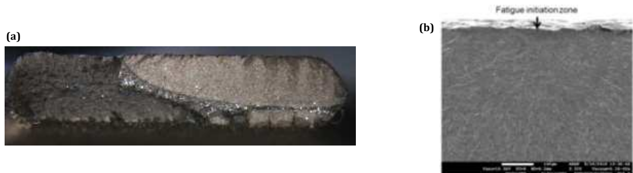
Figure 4: Fatigue fracture surface of the specimen loaded at 600 MPa (R=-1). (a) Global fracture surface showing the fatigue surface, (b) initiation zone identified at the surface of the specimen.
