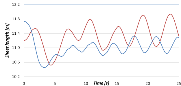
Figure 6 : Result of trimming algorithm on the length of the two gennakers sheets (red line: gen. A, blue line: gen. B): variations showing the instability of the gennakers.
