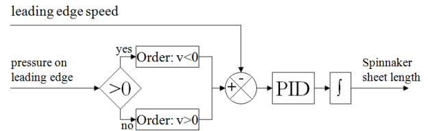
Figure 5 : The trimming algorithm.
