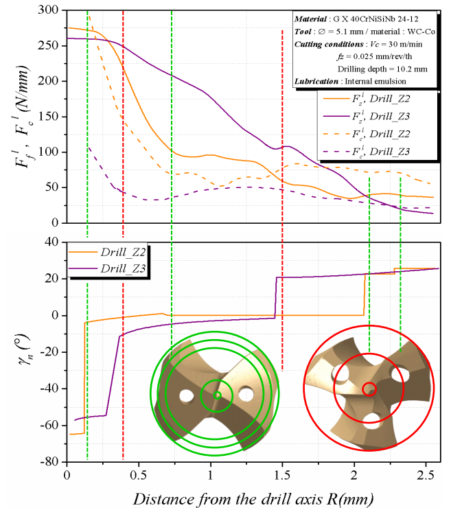
Fig. 4. Linear feed force and cutting force respectively F_f^l , F_c^l correlation with the rake angle \gamma_n taken in normal plan. ( P_n )
