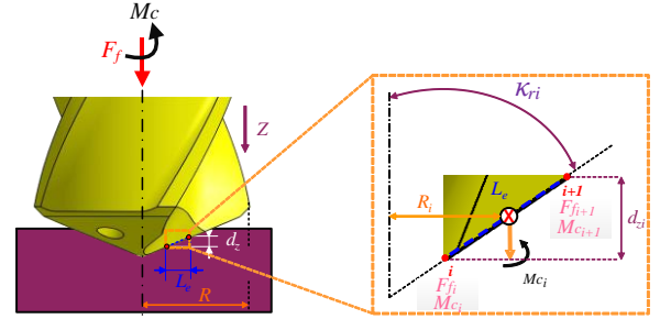
Fig. 3. Principle of the cutting edge discretization during drill tip penetration.
