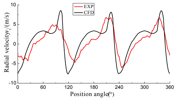
Figure 13 The radial velocity for radius R=370\text{mm}
