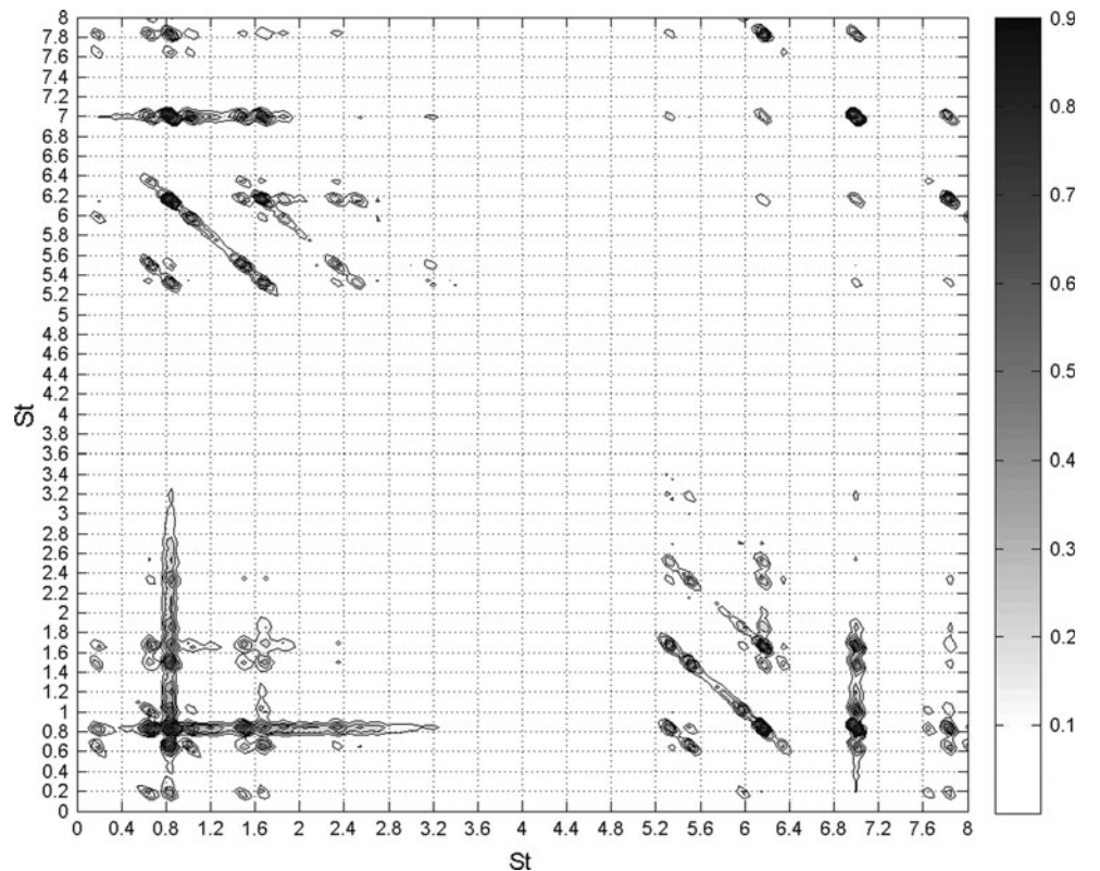
Fig. 5 Bi-coherence of the pressure signals acquired by the microphones located in the diffuser for Q/Q_{des} = 0.26
