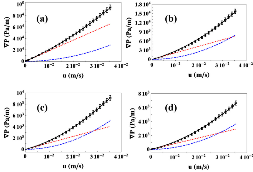
Fig. 1. Pressure gradient vs. average velocity for water injection through the packs of glass beads with (a) d_s = 1 \text{ mm} , (b) d_s = 3 \text{ mm} , (c) d_s = 4 \text{ mm} and (d) d_s = 5 \text{ mm} . Symbols represent experimental data, black solid lines represent their fit to Forchheimer's law, red dotted lines represent the linear term (Darcy's law), blue dashed lines represent the contribution of the quadratic term to the total pressure loss. (For interpretation of the references to color in this figure legend, the reader is referred to the web version of this article.)
