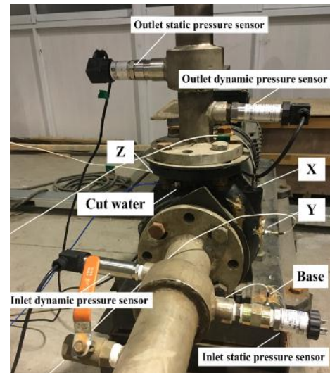
Fig.2 Sensor locations
