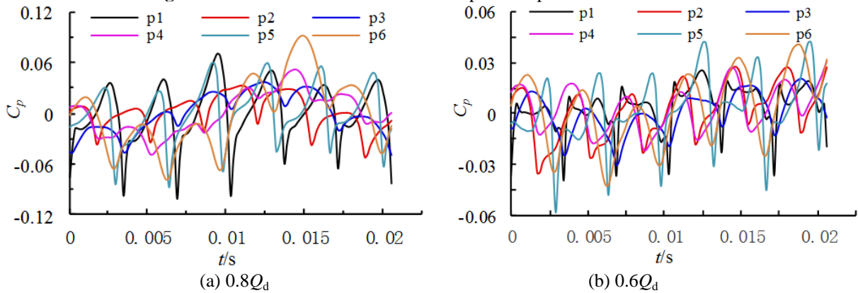
Fig.11 Time domain characteristics of the pressure pulsation at \alpha=7\%
