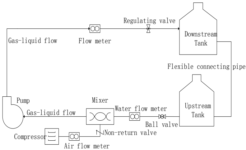
Figure 1: Test rig
