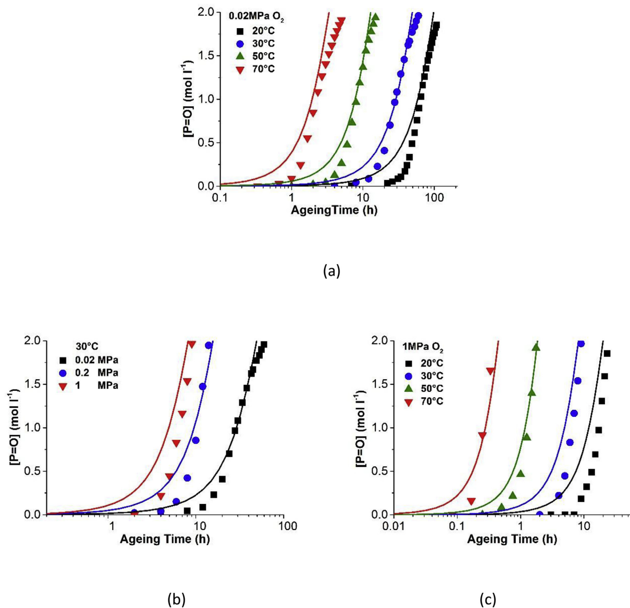
Fig. 11. Variation of the carbonyl concentration as a function of the exposure time, for different ageing conditions of PDCPD: in air, at different temperatures (a); at 30°C, under different oxygen pressures (b) under 1 MPa oxygen pressure, at different temperatures (c).
