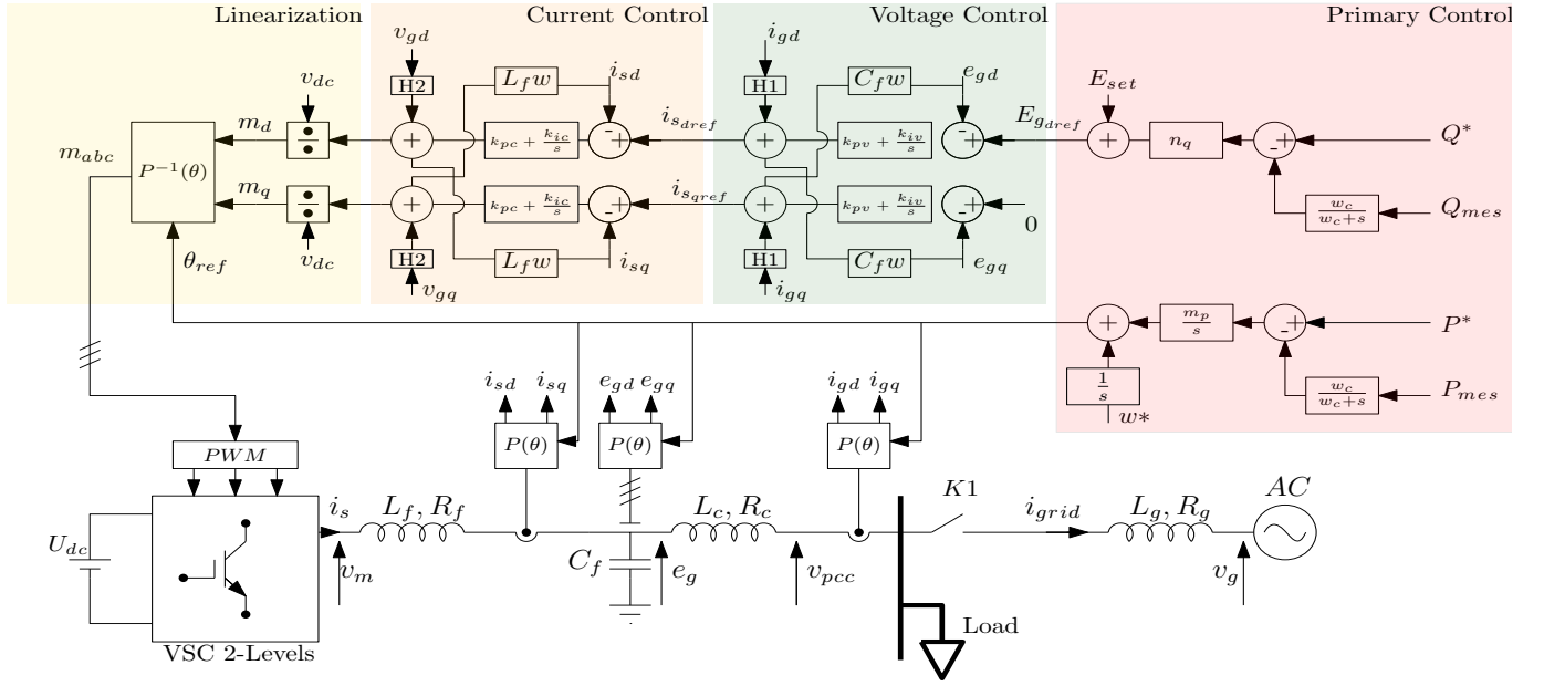
Figure 1. Grid-forming Control
