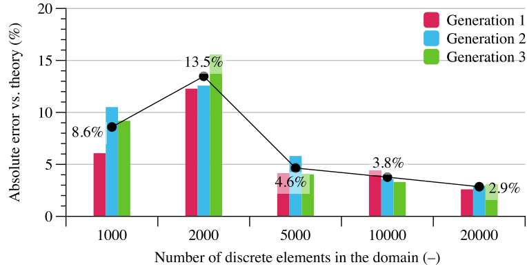
Figure 7. Validation results obtained for a uniform electrical field.
