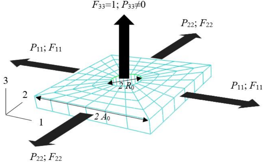
Fig. 6. Initial unit cell used for the comparisons with Tvergaard's results.
