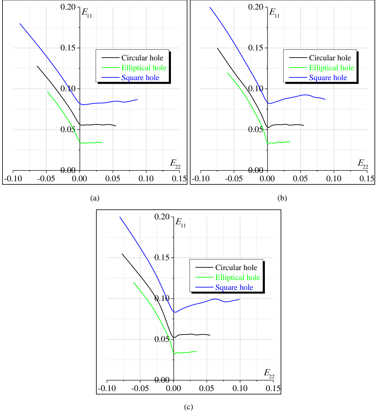
Fig. 16. Effect of the hole shape on the FLDs predicted by: (a) MFC; (b) GBC; (c) RBC.
