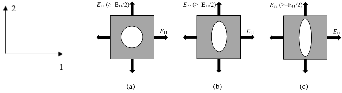
Fig. 11. Unit cells with different elliptical hole initial aspect ratios: (a) b_0 / a_0 = 1 ; (b) b_0 / a_0 = 2 ; (c) b_0 / a_0 = 3 .
