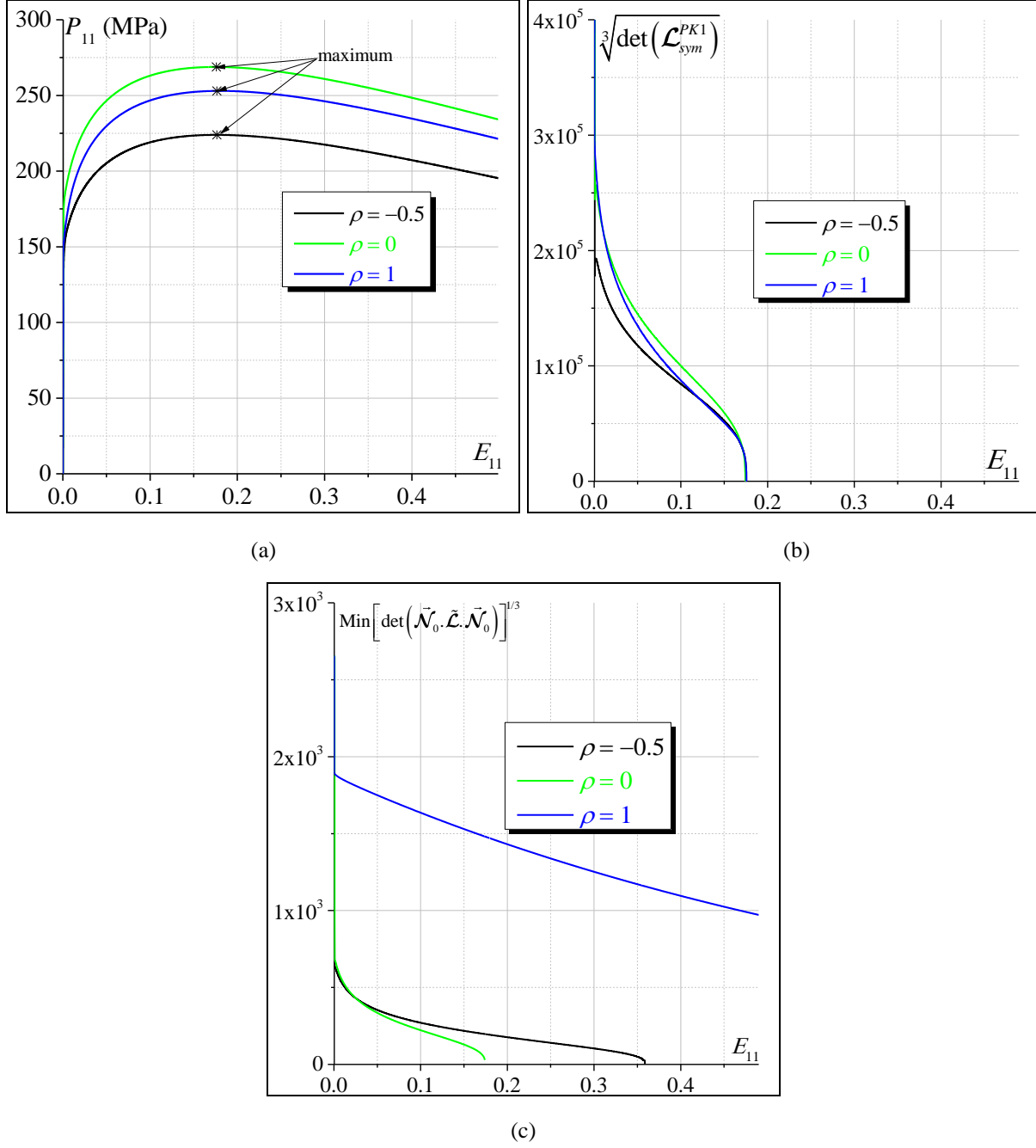
Fig. 4. Prediction of necking, for three particular strain-path ratios, using the different necking criteria: (a) MFC; (b) GBC; (c) RBC.
