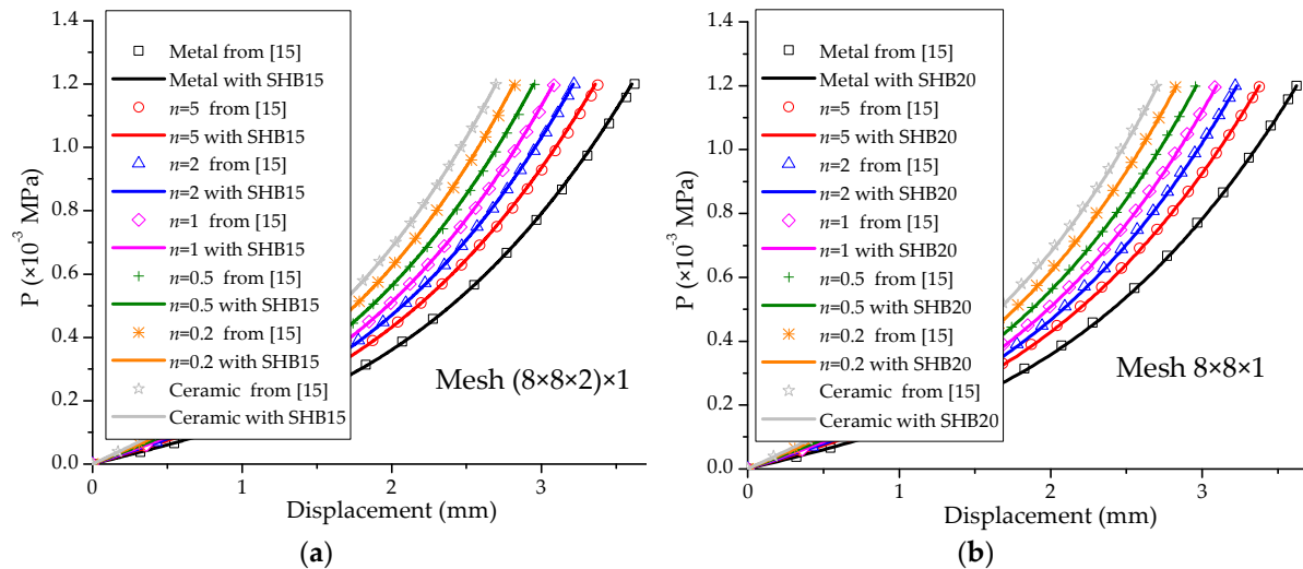
Figure 10. Load–deflection curves at the center point for the square plate. (a) Prismatic SHB15 element; (b) hexahedral SHB20 element. Please add a white space before/after = and \times in images.
