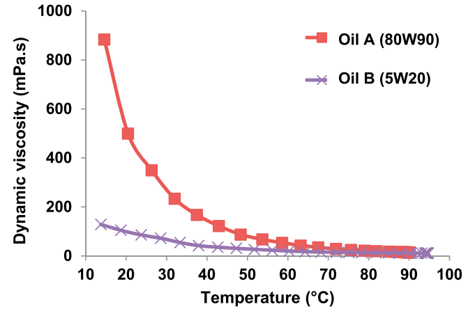
Fig. 6. The dynamic viscosity functions of temperature of the two considered oil.
