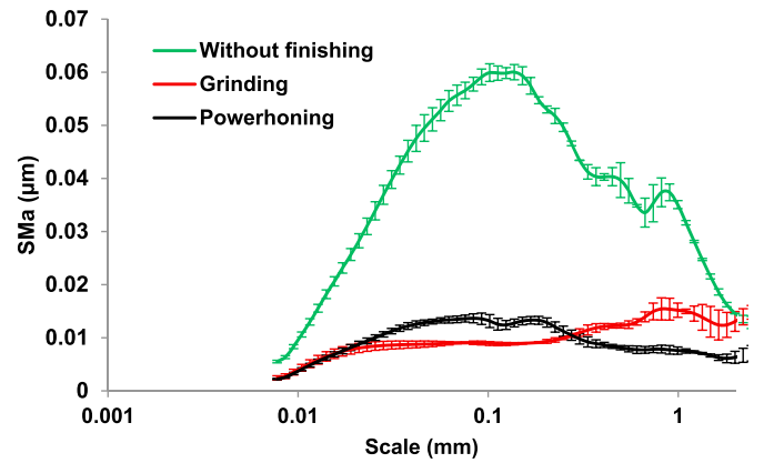
Fig. 3. Example of surface roughness spectra for three considered gears surface finishes before gear testing.
