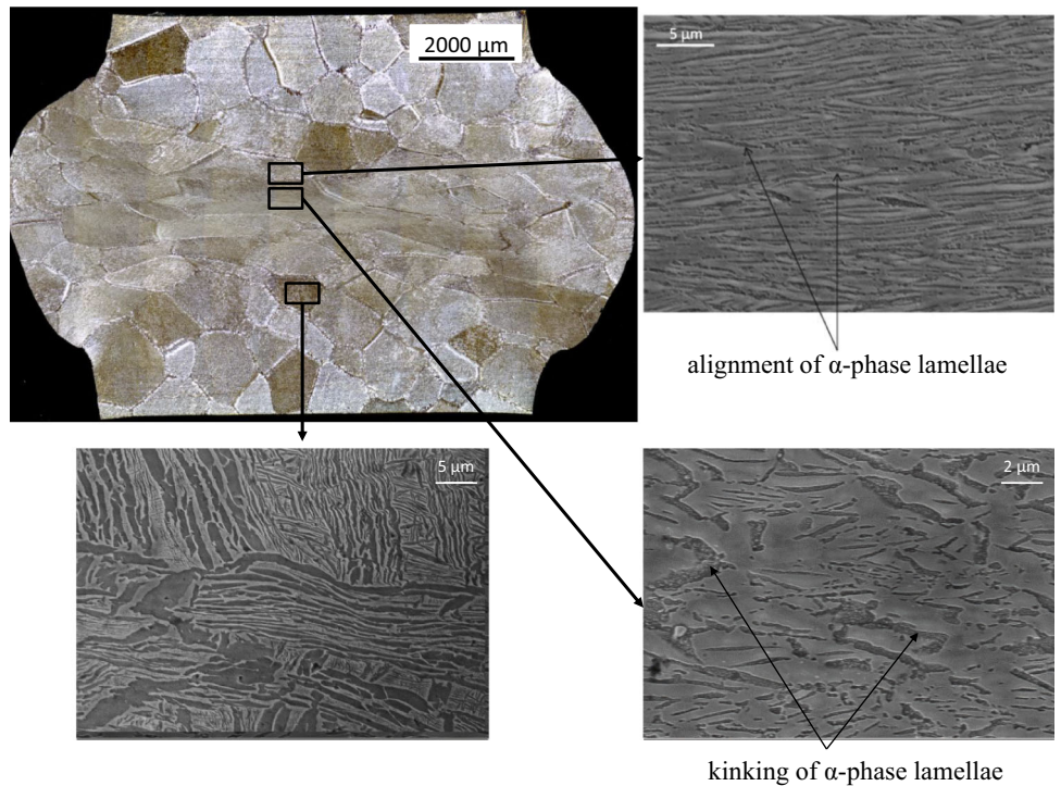
Figure 9 SEM observations of a Ti17 specimen after deformation at a strain rate of 1 \text{ s}^{-1} and a temperature of 750 °C: alignment of \alpha -phase lamellae and kinking of \alpha -phase lamellae. The compression axis is vertical.
