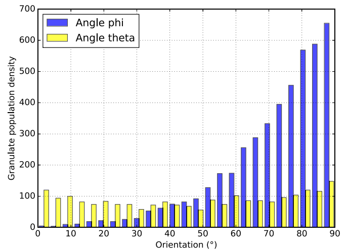
Fig. 9. Orientation of cork granulates obtained through X-ray microtomography.
