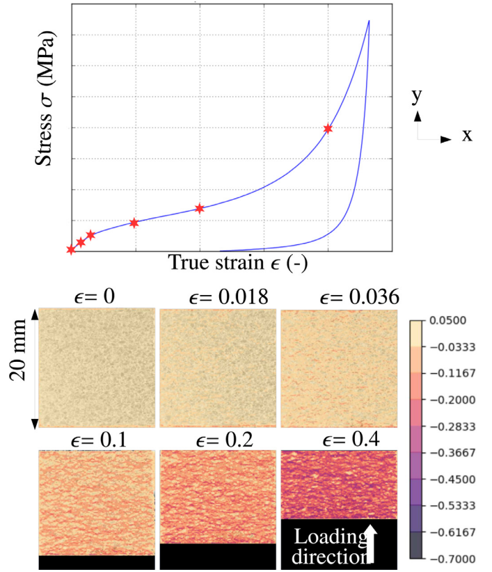
Fig. 21. YY-Strain map at several moments of the compression of cork agglomerate in the out-of-plane direction at 5 \text{ mm min}^{-1} .
