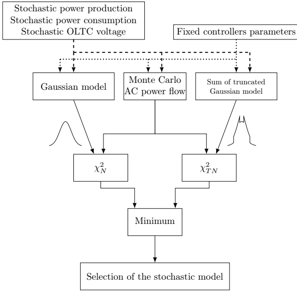
Fig. 4. Flowchart of the selection algorithm
