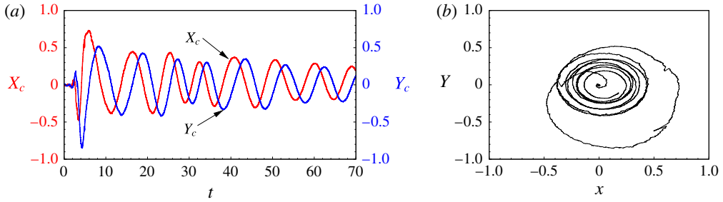
FIGURE 15. (Colour online) Results for Re=5000 isolated vortex: (a) displacement of the vortex centre with time for computations initiated with the T=4.8 , E(0)=0.01 nonlinear optimal perturbation; (b) trajectory of the vortex centre in the vortex plane.
