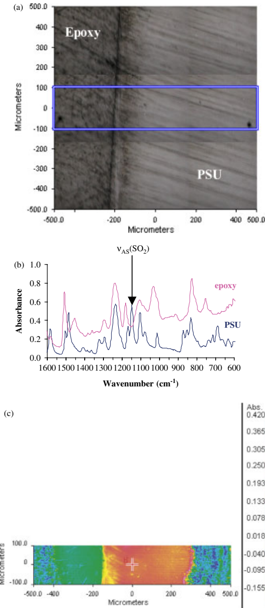
Figure 1. Profiles obtained using ATR microscopy. (a) Image of analysed sample at the PSU–epoxy interface. (b) FTIR spectra of epoxy and PSU. (c) Localization of PSU sample using 1145 cm -1 absorption. One sees the ‘edge effect’ preventing analysis of the regions of the x-axis of x < -400 \mu\text{m} or x > 400 \mu\text{m} .
