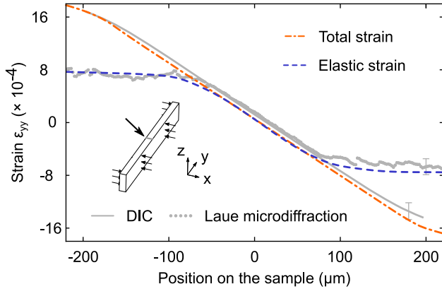
Fig. 2. Elastic and total (i.e., elastic + plastic) strain evolution across the thickness of a [100] bent single crystal. The positions of measurement points are along x direction on the surface normal to z (inset). Experimental data from DIC and Laue microdiffraction (grey curves) are compared with the identified crystal plasticity model (blue and red curves) (Color figure online).
