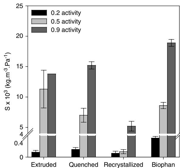
Figure 4. Apparent solubility coefficient ( S ) of ethyl acetate in PLA samples with varying crystallinity at three activities ( p/p_0 ) at 25 °C. In order to display the small values, the ordinate is discontinuous as indicated.
