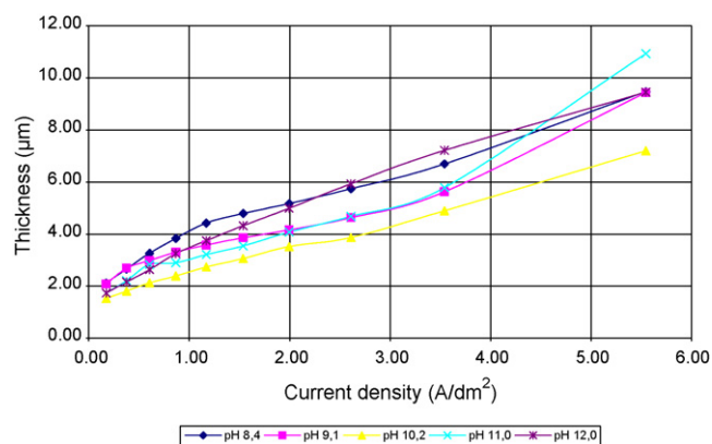
Fig. 7. Effect of pH of the plating bath (temperature = 70 °C, [\text{Sn}^{4+}] = 58.8 \text{ g L}^{-1} , [\text{Zn}^{2+}] = 7.23 \text{ g L}^{-1} ) at variable current density on the thickness of the tin-zinc alloy coating.
