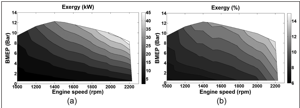
Figure 7. Exergy of the exhaust gases: (a) in kilowatts; (b) in percentages of the fuel energy. BMEP: brake mean effective pressure; rpm: r/min.
