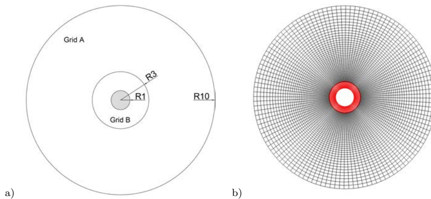
Fig. 15 Supersonic flow over a cylinder with static configuration. a) Geometry description and b) non-conformal grids.
