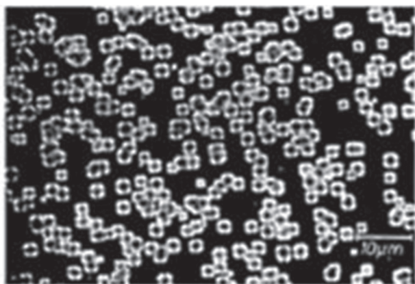
Figure 6. Optical microscopy photo of pure PPS at T_c = 221\text{ }^{\circ}\text{C} . Adapted with permission. [75] Copyright 1994, Wiley-VCH.
