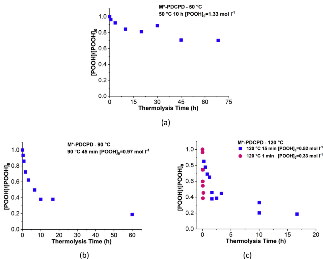
Fig. 4. Changes in normalized hydroperoxides concentration ( [\text{POOH}]_0 is the hydroperoxide concentration after ageing under air – see Fig. 2) for thermolysis of M^* -PDCPD at 50 (a), 90 (b) and 120 °C (c). NB: time to totally destroy POOH at 50 °C was too long so that thermolysis were interrupted after 70 h.
