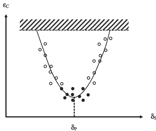
Figure 21.5 Shape of the variation, against parameter of solvent solubility ( \delta_S ), of critical strain ( \varepsilon_C ) for PPO [5]. Minimum of curve corresponds to: \delta_S = \delta_P , \delta_P being the parameter of polymer solubility. (○) crazes; (●) open cracks.
