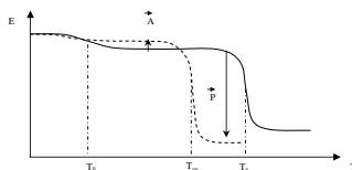
Figure 5.27. Shape of the modulus variation with temperature in the case of an unplasticized polymer (continuous line) and plasticized (dotted line). T_g \sim T_g'
