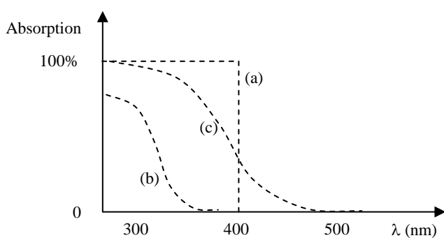
Figure 7.22. Absorption spectrum of UV absorbers: (a) ideal UV absorber; (b) UV absorber with limited protective power but colorless; (c) efficient UV absorber but yellow (it absorbs at \lambda > 400 nm in violet)
