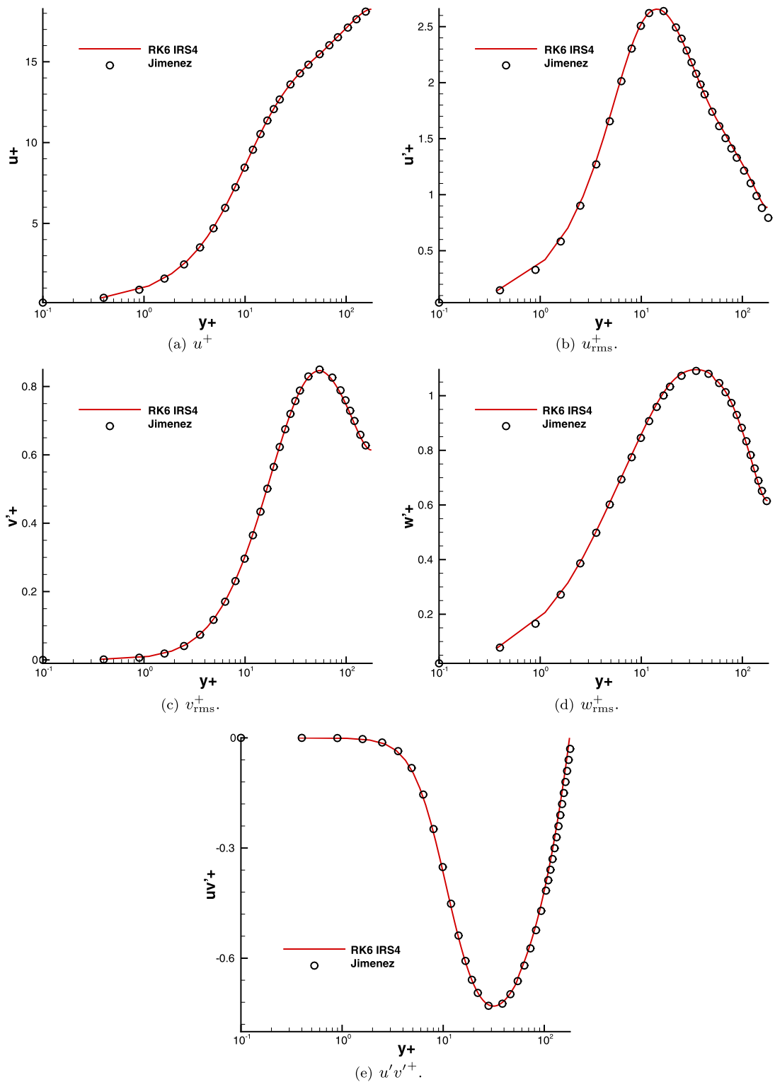
Fig. 26. Quasi-incompressible turbulent channel flow. Computed (\cdot)^+ profiles for RK6IRS4 at CFL_0 = 5 .
