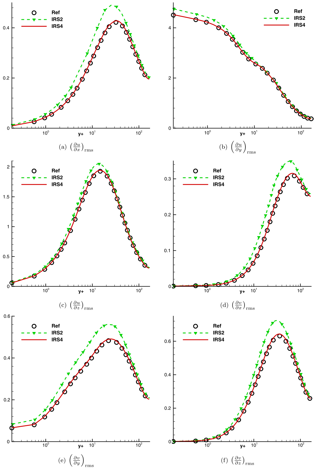
Fig. 28. Compressible turbulent channel flow. Computed (\cdot)_{rms} profiles of the velocity gradients for RK6IRS2 and RK6IRS4 at CFL_0 = 5 compared to RK6 predictions at CFL_0 = 1 (reference) [first part].
