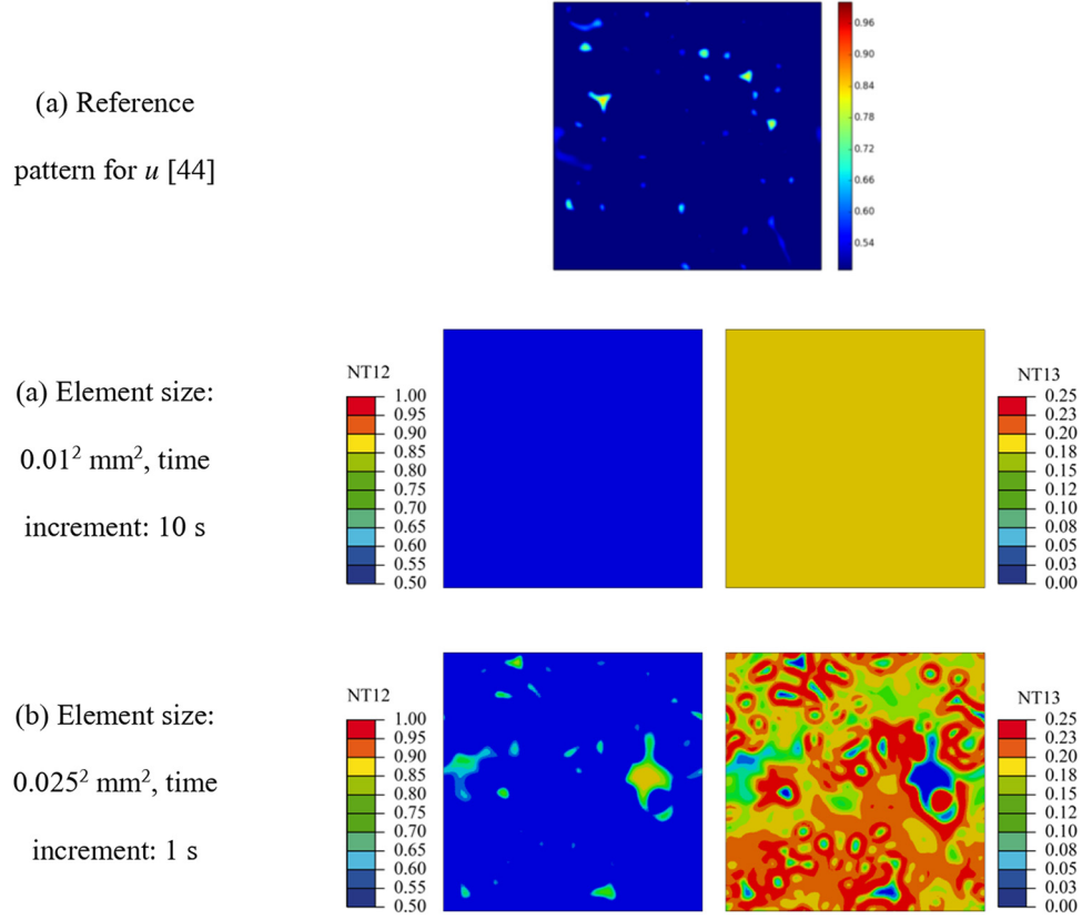
Fig. 10. Influence of the time increment on the Abaqus results at t=5000 s for u (left) and v (right), with (F,k) = (0.022, 0.049) .
