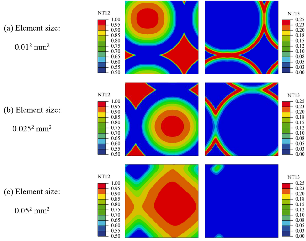
Fig. 9. Influence of the element size on the Abaqus results at t=800 s for u (left) and v (right), with (F,k) = (0.006, 0.037) .
