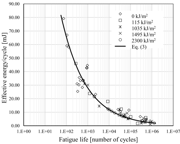
Fig. 14. Effective dissipated energy per cycle versus fatigue life (markers: experimental data, continuous lines: Eq. (3)).
