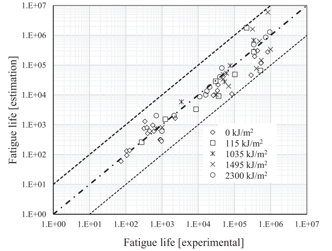
Fig. 15. Comparison between predicted and experimental fatigue life results using the modified Ostrohmeyer model.
