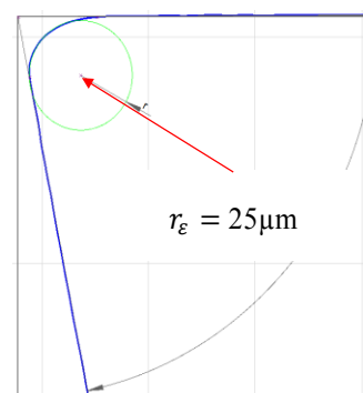
Fig. 1. Measurement of the edge radius
