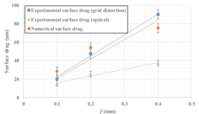
Fig. 7. Variation of surface drag against feed
