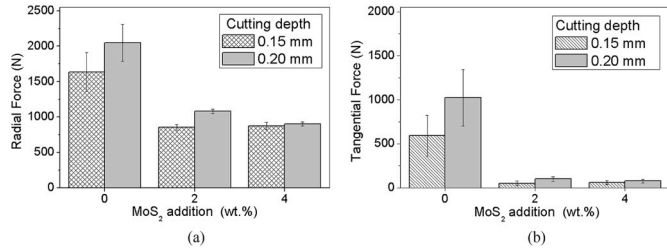
Fig. 10. Effect of the MoS 2 addition in orthogonal cutting at different depths ( d ) on average force signals (a) radial and (b) tangential.
