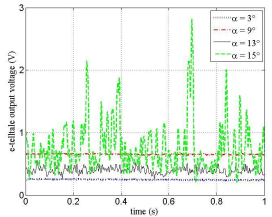
Figure 8: Time series of the e-telltale output voltage for \alpha = 3^\circ , 9^\circ and 15^\circ .
