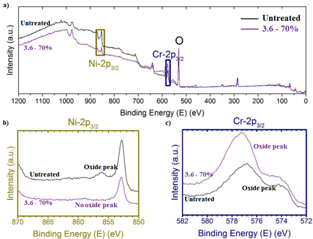
Fig. 10. XPS Spectra of untreated surface and laser treated surface at 3.6 \text{ J/cm}^2 laser fluence and 70% overlap : a) overview of the spectra, b) zoom on the (Ni) oxide peak, c) zoom on the (Cr) oxide peak.
