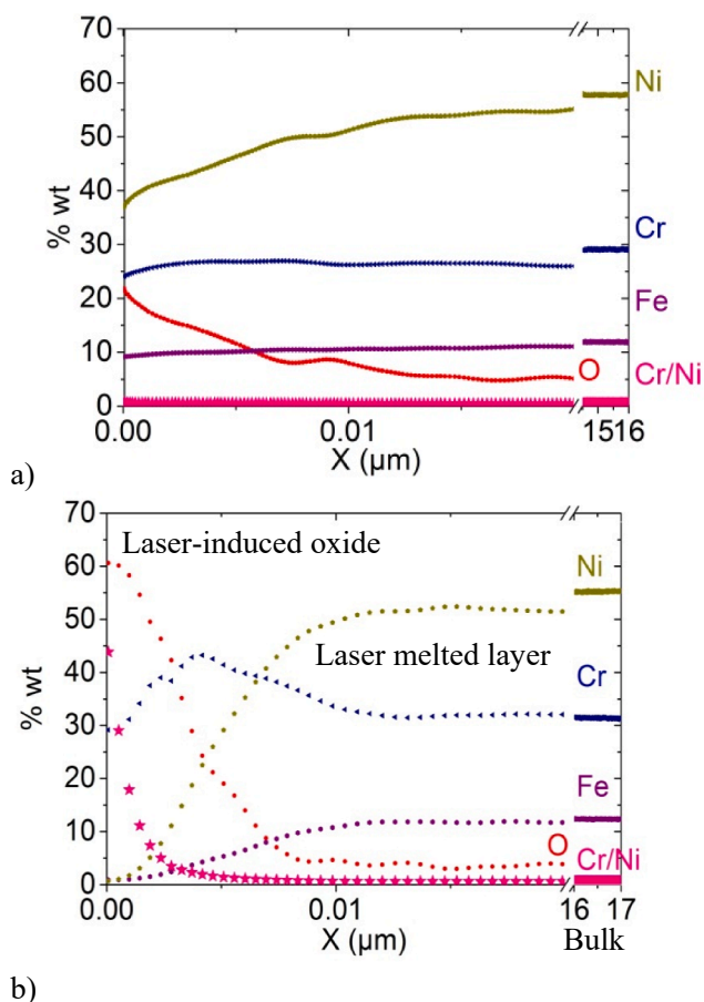
Fig. 7. GDOES chemical composition profiles along depth for Ni, Cr, Fe, and O and the ratio of the Cr content over the Ni content. The dimensionless Cr/Ni values should be read using the labels on the vertical axis. a) Raw surface. b) Laser treated surface (treatment conditions: 3.6 J/cm 2 and 70% overlap).
