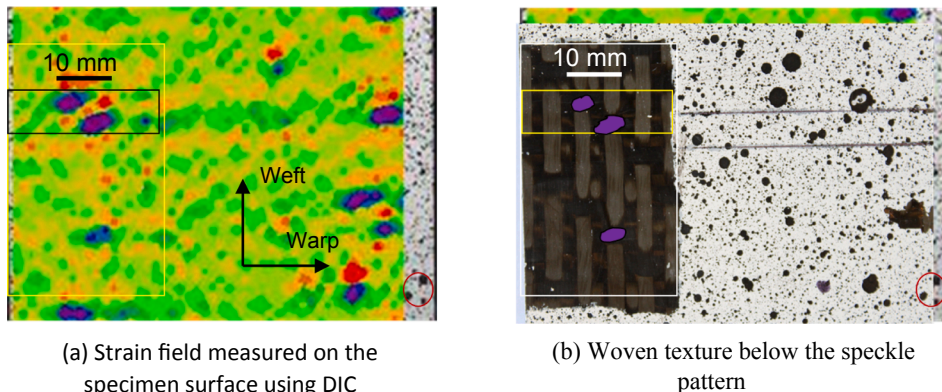
Fig. 7. Correlation between the weaving pattern and the high strain concentration areas.
