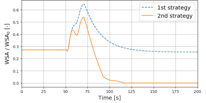
(f) Relative value of main hull wetted surface area.
