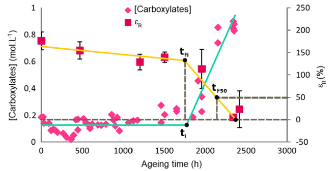
FIGURE 6 Comparison of the thermal oxidation and embrittlement kinetics in XLPE-C in air at 150 ^{\circ}\text{C}
