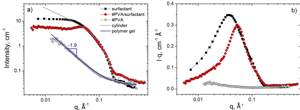
Fig. 2. The scattering curves in I(q) (a) and I \cdot q(q) (b) coordinates for #PVA/potassium oleate/ C_8 TAB system cross-linked with borate (red diamonds) and its components: potassium oleate/ C_8 TAB solution (black squares) and #PVA (grey circles) in D_2O . Concentrations: 4 wt% PVA, 2.5 wt% potassium oleate, 0.8 wt% C_8 TAB, 0.018 M potassium borate (molar fraction of borate with respect to PVA repeat units – 0.02). Grey line is a fit of the scattering curves by a form-factor of cylinder with radius R = 18.6 \pm 0.2 Å. Blue line is a fit of the scattering curve by a generalized Ornstein-Zernike (gel) model with mesh size \xi = 26 nm and fractal dimension D = 2.06 .
