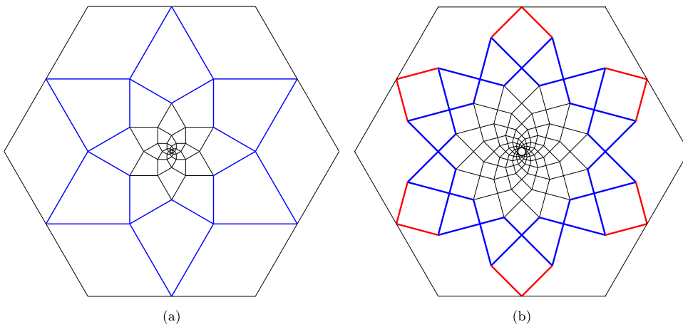
Fig. 9. Slip line fractal networks for the hexagonal cells. (a) H0 cell and (b) H15 cell.
