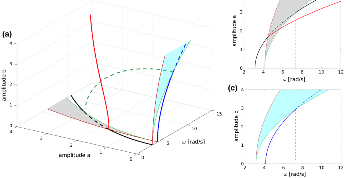
Fig. 3 a Three-dimensional representation of the solution branches in the (\omega, a, b) space. Black line: backbone of the A-mode, blue line: backbone of the B-mode, red line: elliptic mode, green line: normal mode. Unstable solutions are marked
