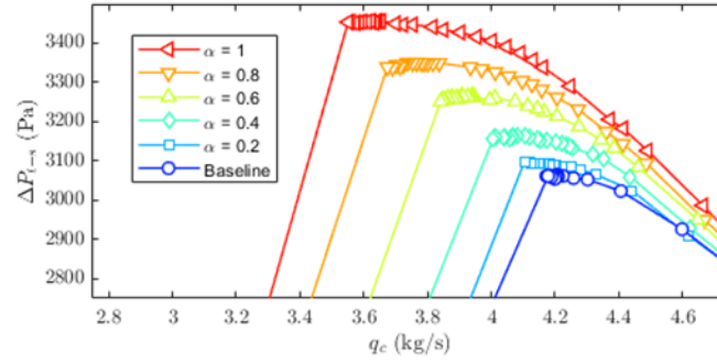
Figure 12: Stability improvements achieved on the compressor performance map by using the pulsed jets control system with various duty cycle values ( p = 7.5 bar, f = 100 Hz and 20 injectors activated)
