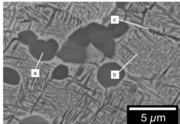
Figure 2 BSE SEM image showing the typical microstructure of the as-received state of Ti-5553 titanium alloy. (a) nodular \alpha phase, (b) fine lamellar \alpha phase, (c) coarse grain boundary \alpha phase.
